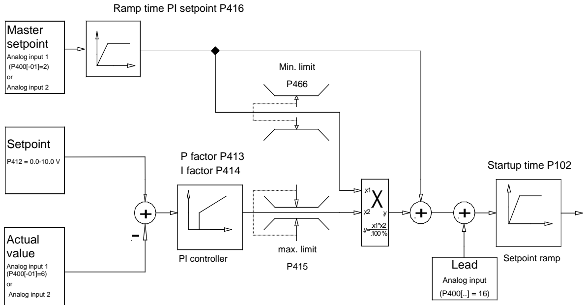
Figure 32: Process controller flow diagram
