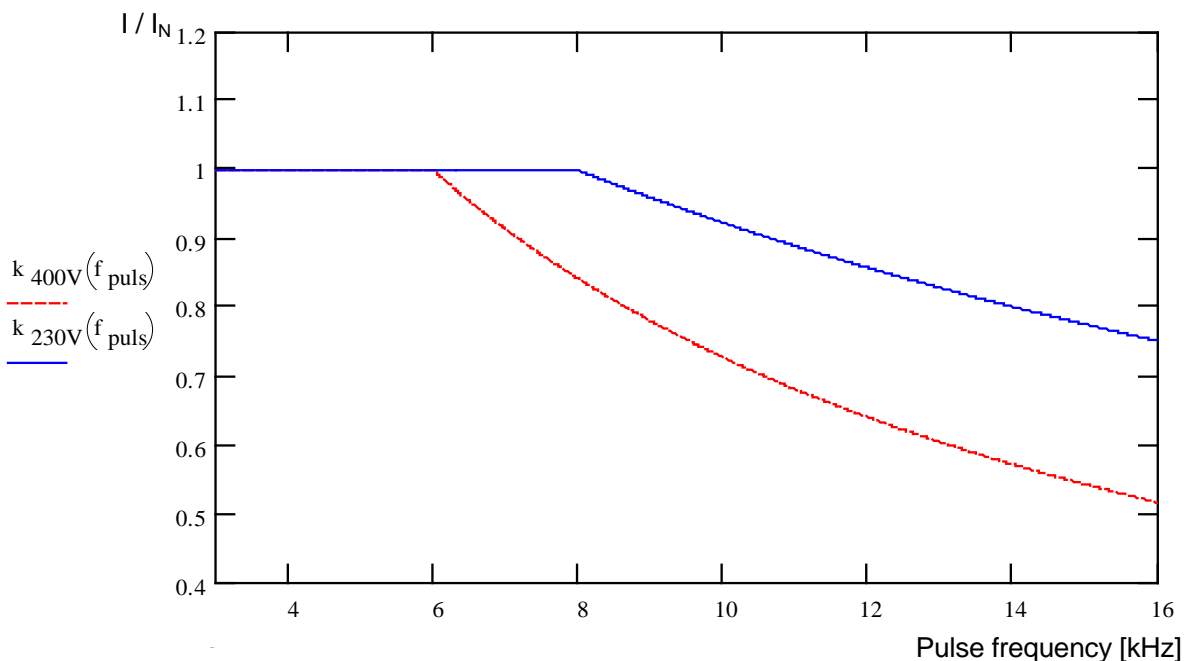
Figure 34: Heat losses due to pulse frequency
