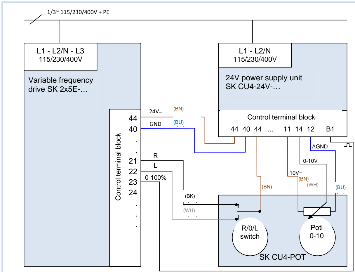
Figure 26: Connection diagram and parameterization of SK CU4-POT, example SK 2x5E
