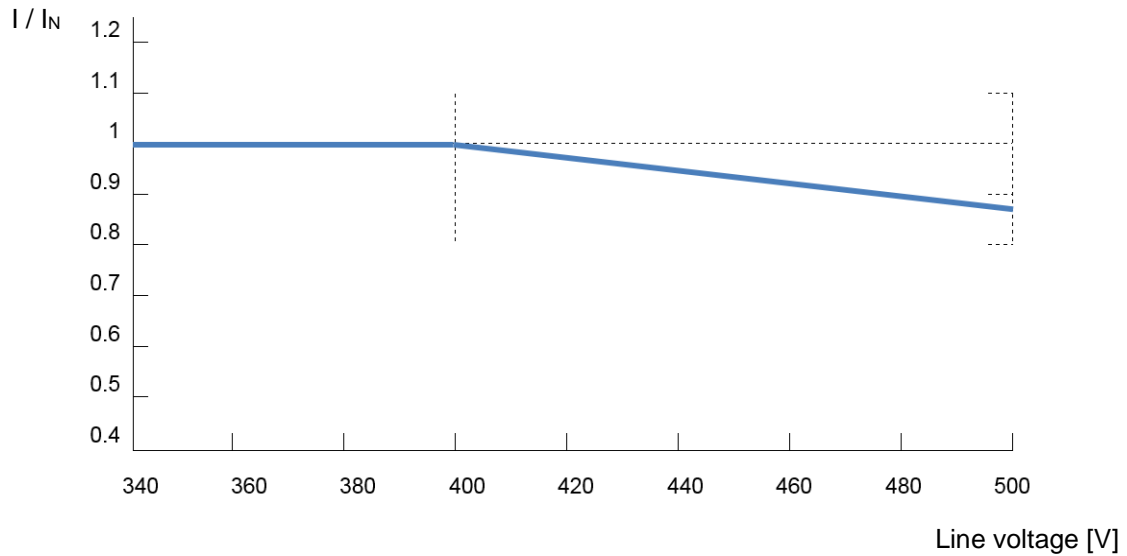
Figure 35: Output current due to line voltage
