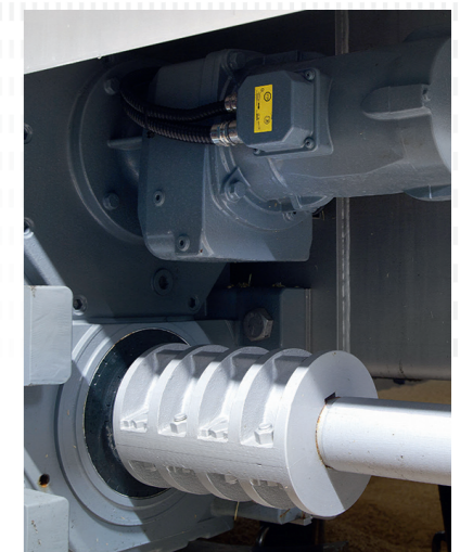
Travelling drive The UNICASE parallel shaft gear unit with helical gear first stage moves the turning machine over the saladin vat.
